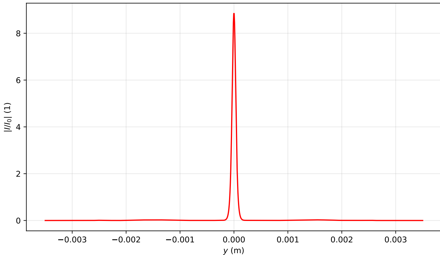
Intensity profile I(x=0, y, z=1.115)/I_0 , \text{Pin}=6.0\text{Pcr} , artificial time
